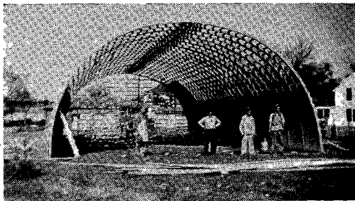
Interior View of Tabernacle Construction, Showing Curved Bows Which Span the Roof
